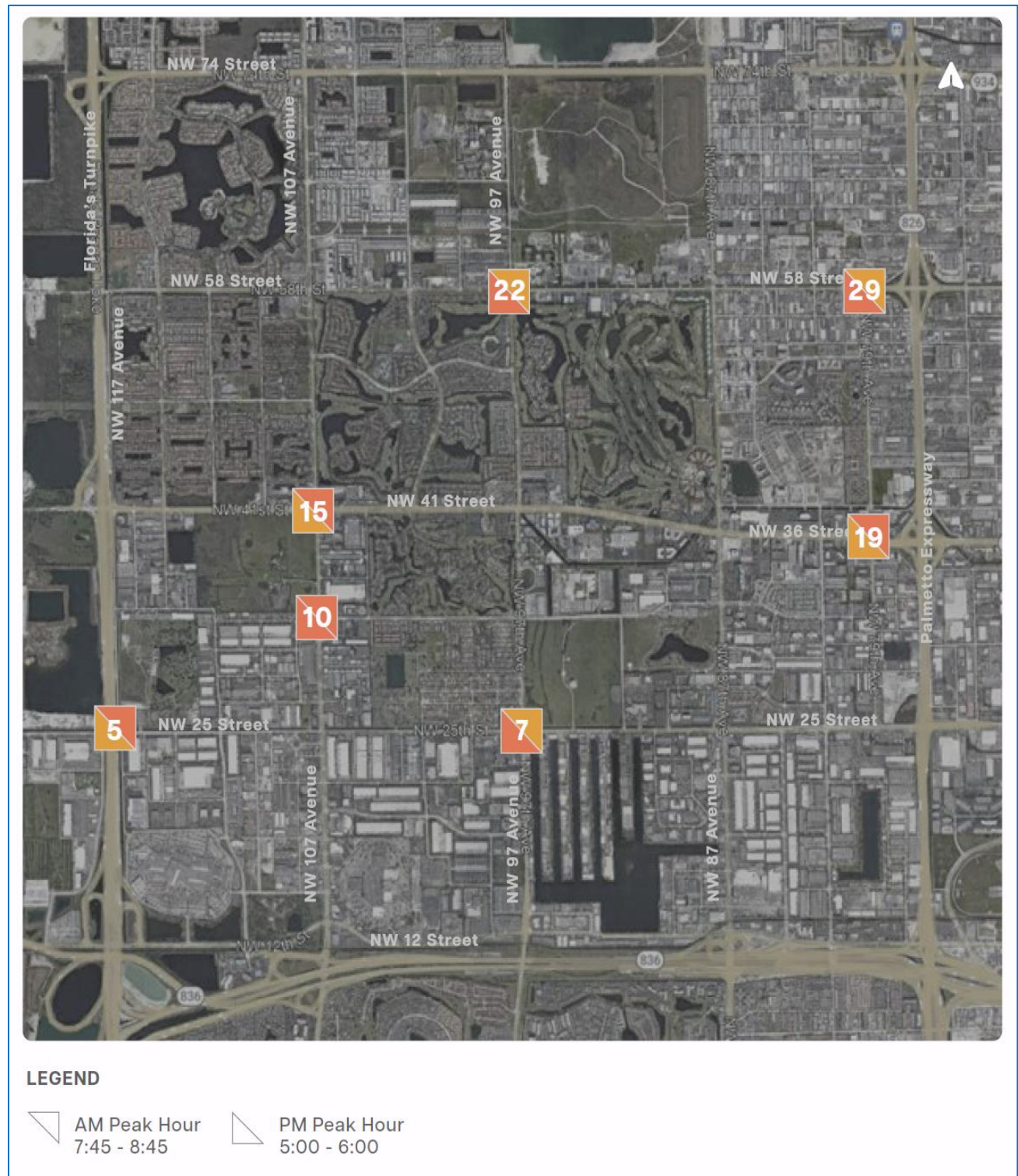
Figure 5. 2023 Failing Intersections
